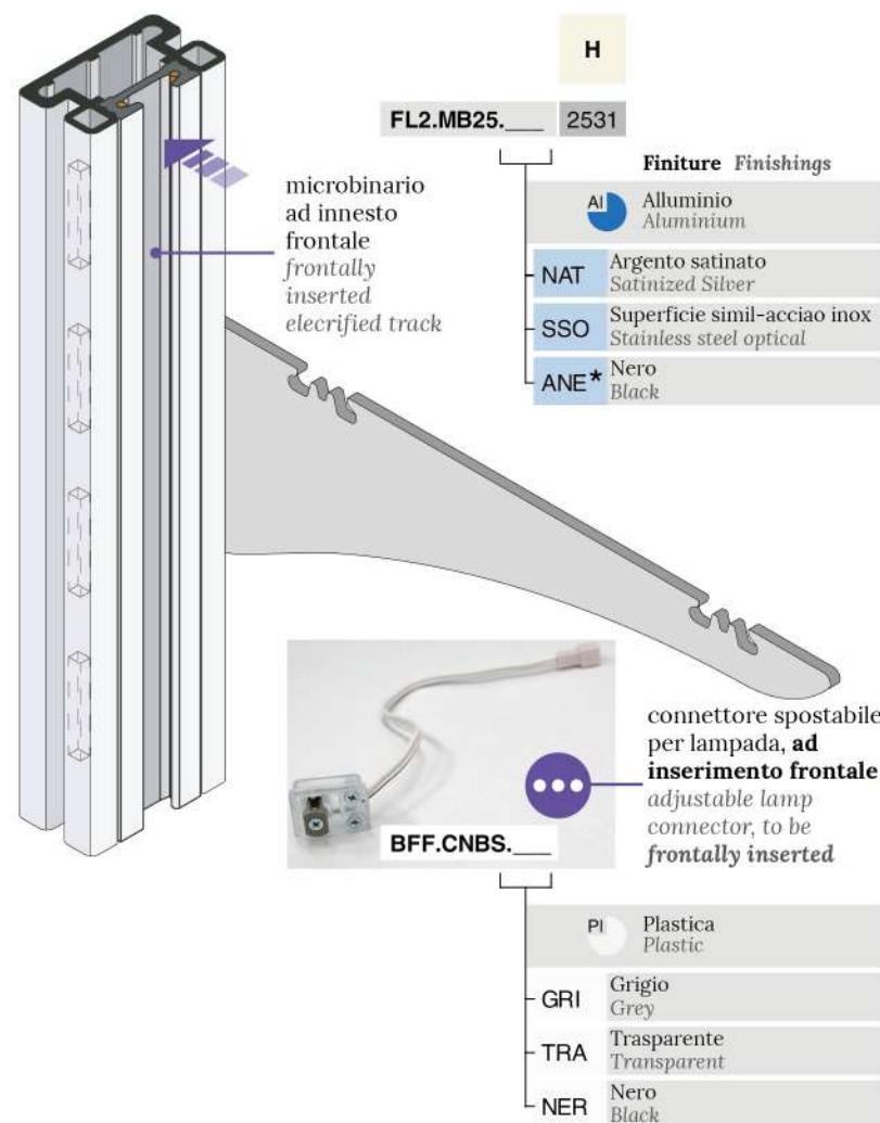
microbinario in finitura abbinata electrified track in matching finishing
